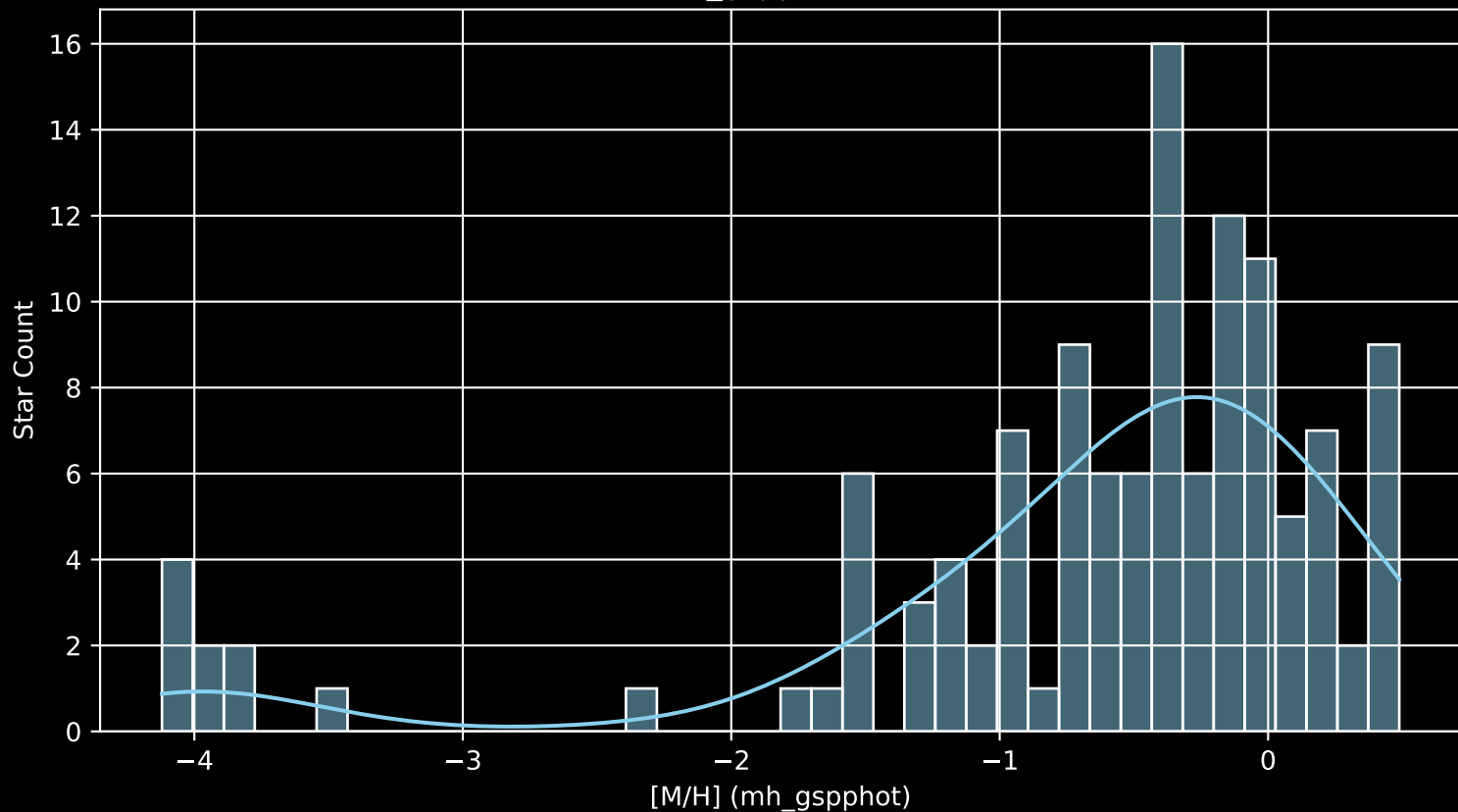
APOGEE DR17 Field: [353+17-O [M/H] (mh_gspphot) (n= 124)
