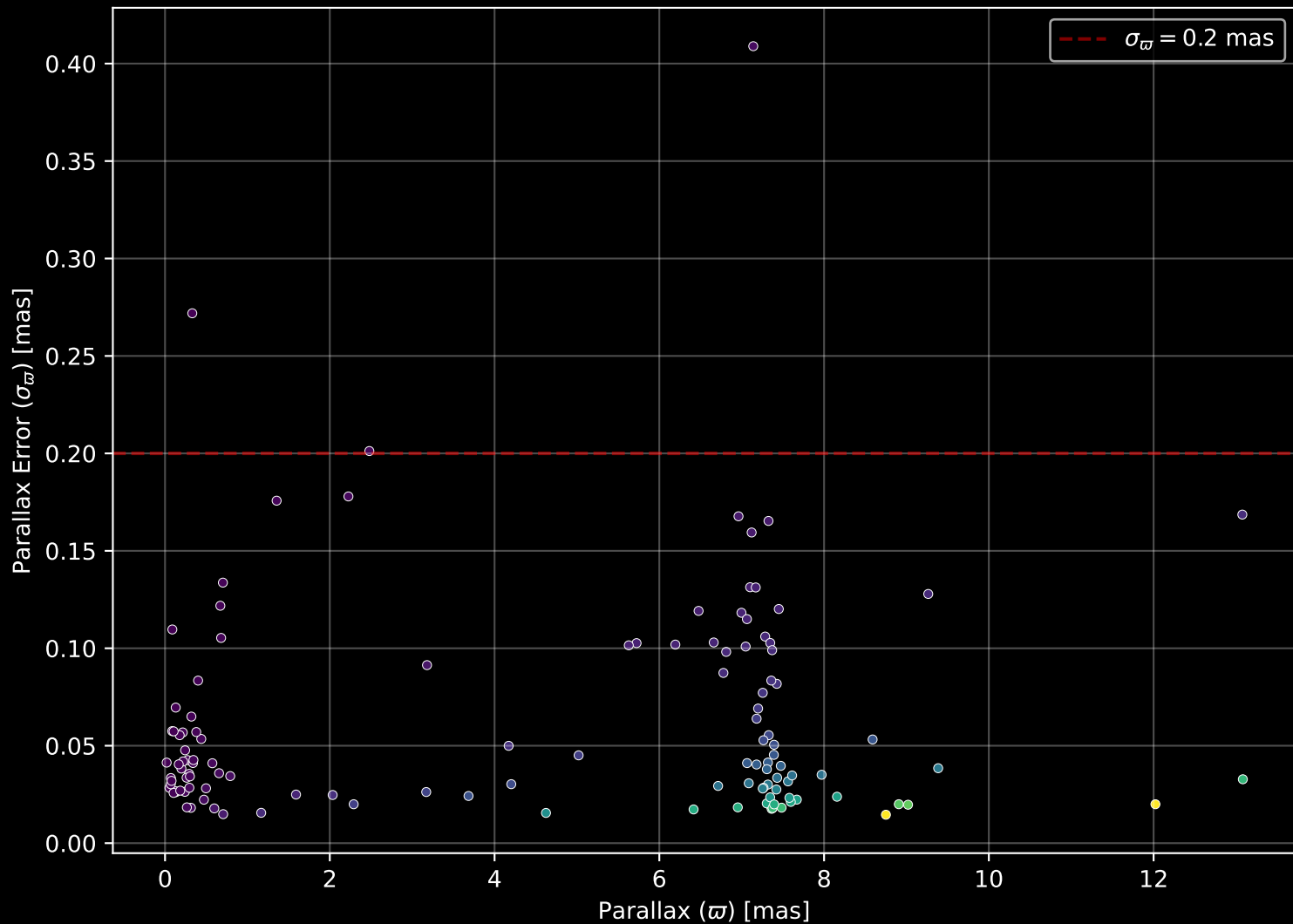
APOGEE DR17 Field: [353+17-O] Parallax Quality (n= 125)
