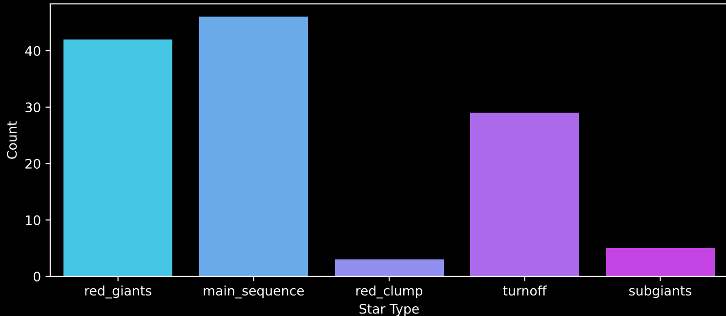
APOGEE DR17 Field: [353+17-O] Count plot of Star Type
