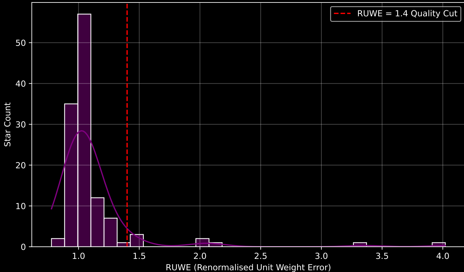
GAPOGEE DR17 Field [353+17-O] RUWE Distribution (n= 122)
