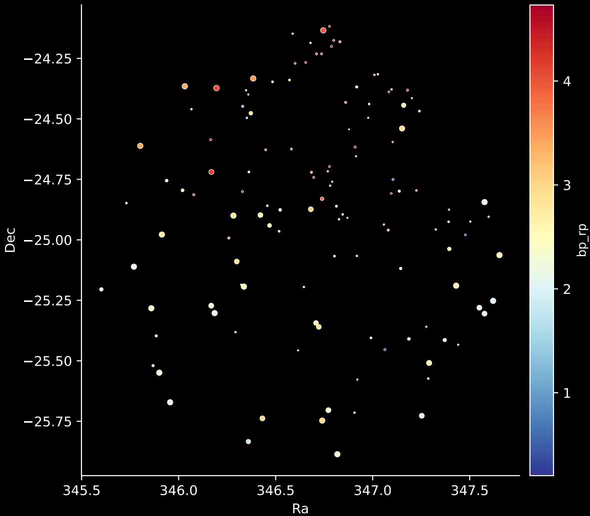
APOGEE DR17 Field: [353+17-O] Stars: 125
