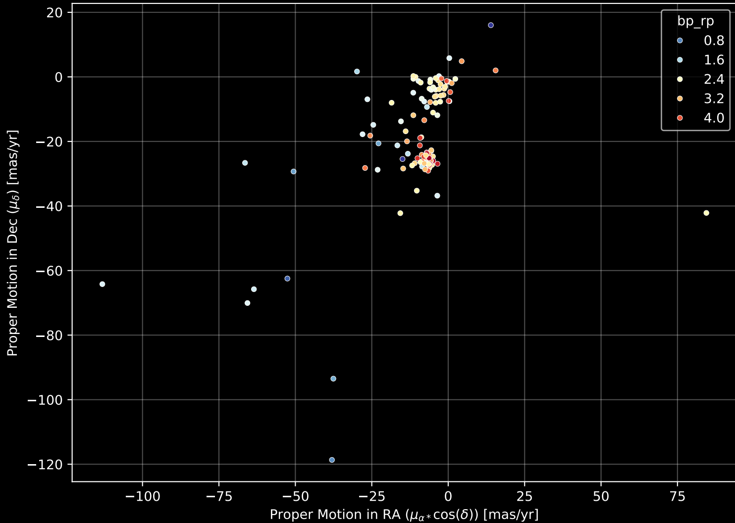
APOGEE DR17 Field: [353+17-O] Proper Motion Diagram (n= 125)
